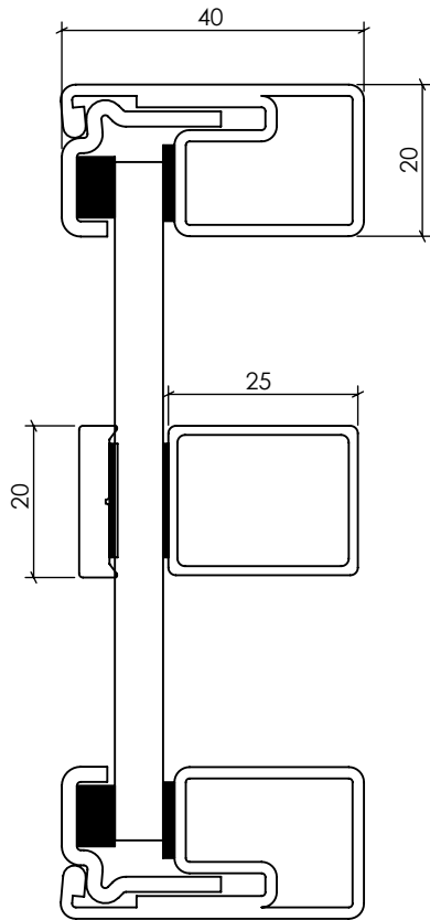
LOFT 20 CONSTRUCTION BAR (WELDED ONE SIDE)
